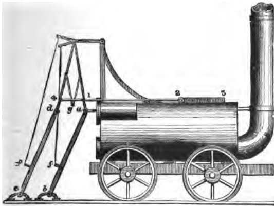
Fig. 4.—"Brunton's Engine," 1813.
